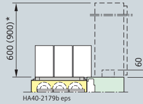
Design option with busbar voltage transformers for all circuit-breaker types
