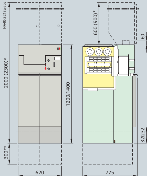
Bus sectionalizer panel/module type S(620) with three-position switch-disconnector and earthing on the right
