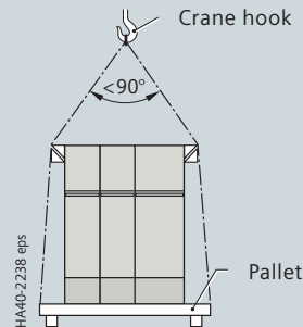
Crane transport with pallet
