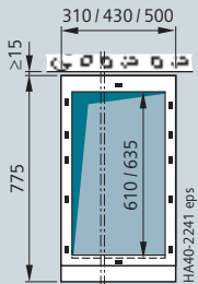
Deep cable compartment cover: Without
