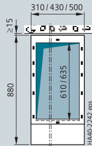
Deeper by 105 mm
