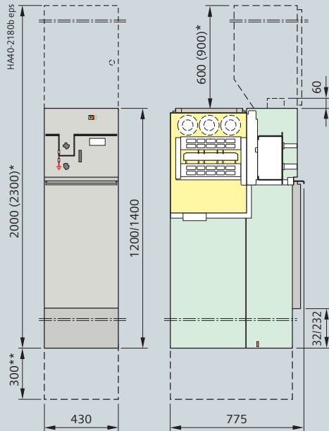
Bus sectionalizer panel/module type S with three-position switch-disconnector and earthing on the left
