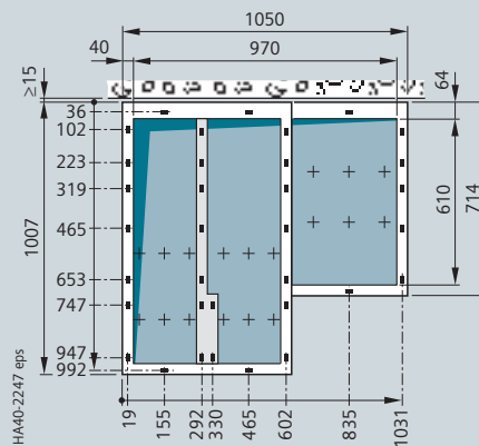
Type RRT deeper by 300 mm
