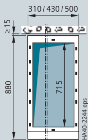
Deep cable compartment cover with base extension: Deeper by 105 mm
